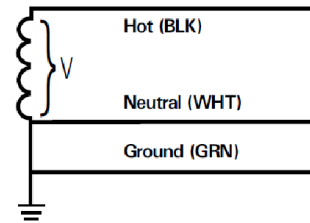
SINGLE POLE 1 Hot, 1 Neu, 1 Grnd
